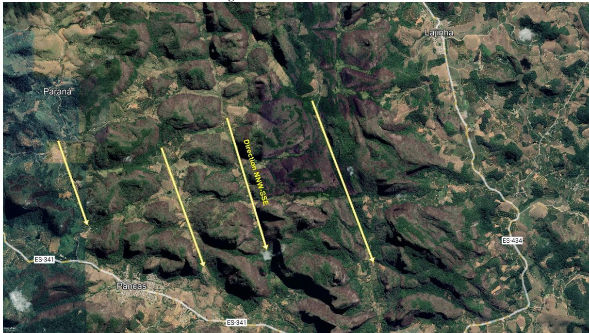
Figure 14 - Linear features
