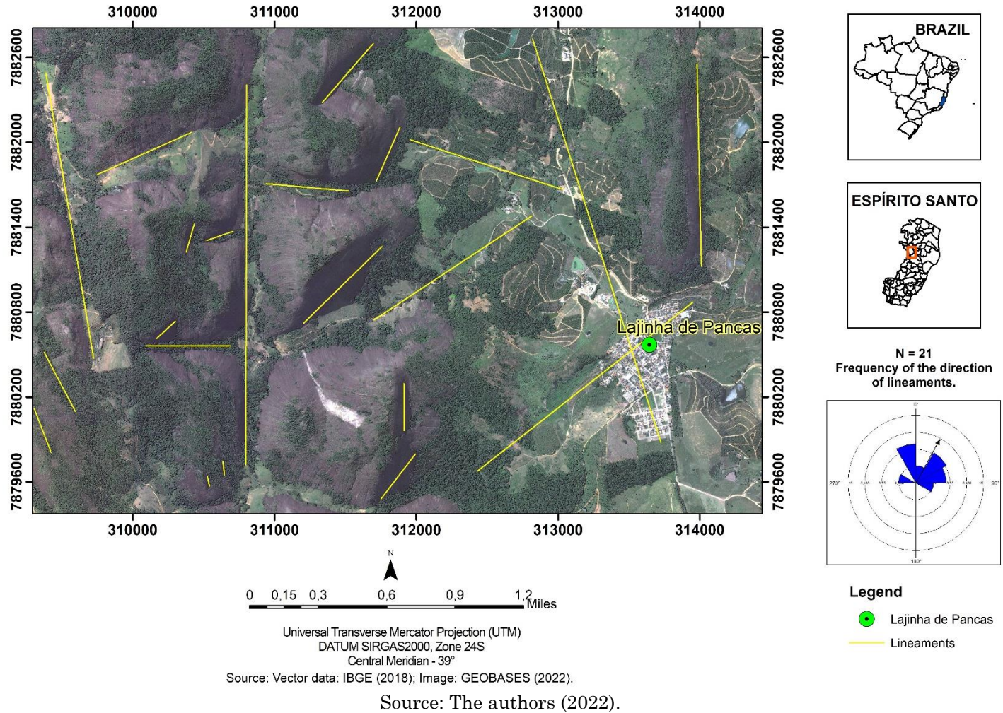
Figure 6 - Lineament map in digital orthophoto - Scale 1:25.000
