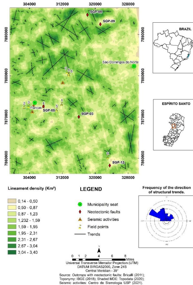
Figure 5 - Lineament density map and structural trends
