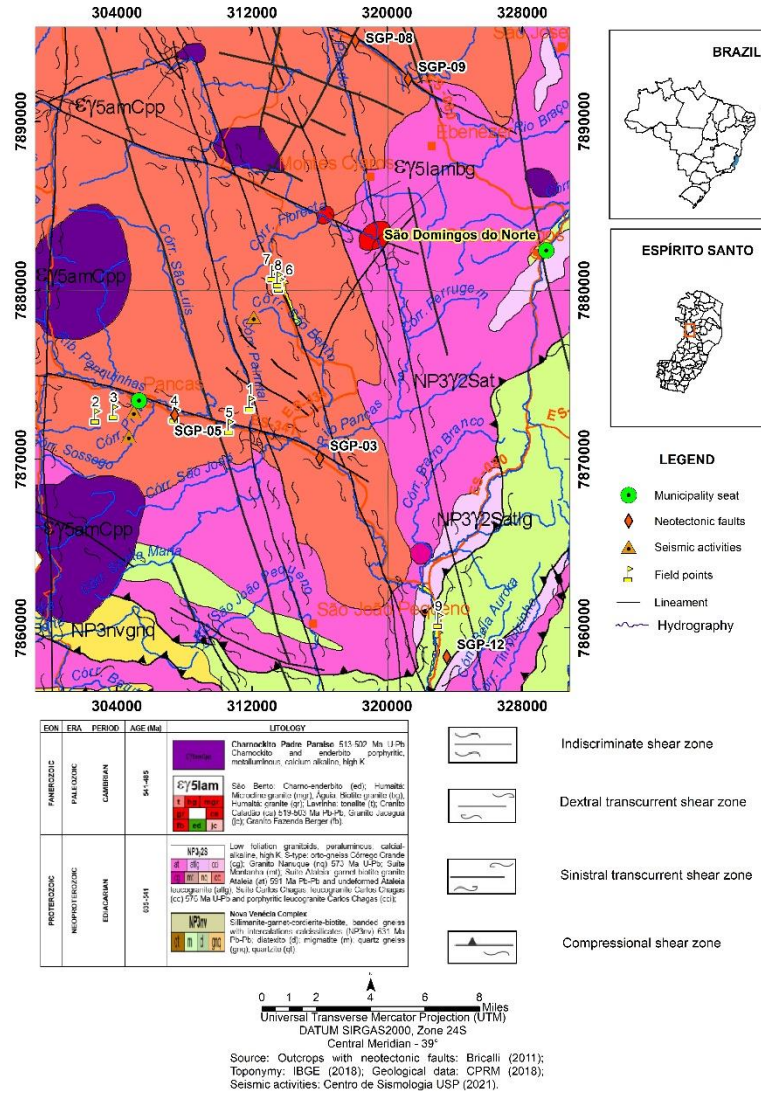
Figure 2 - Geological map of the studied área
