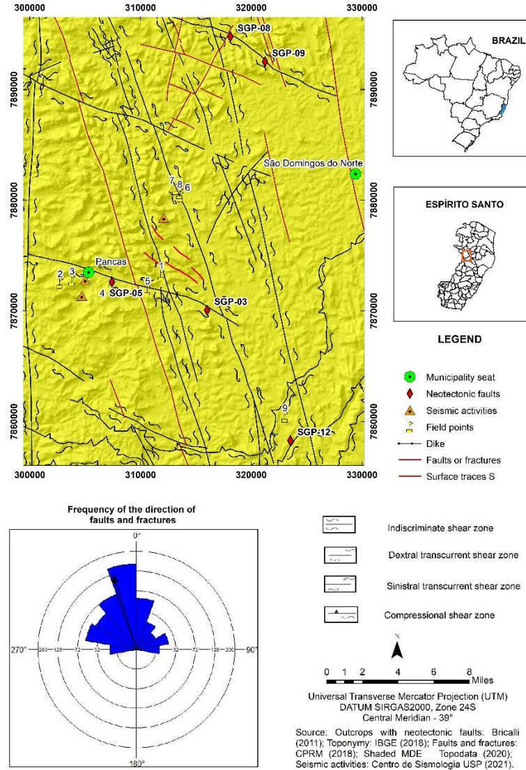
Figure 7 - Fault and fracture map
