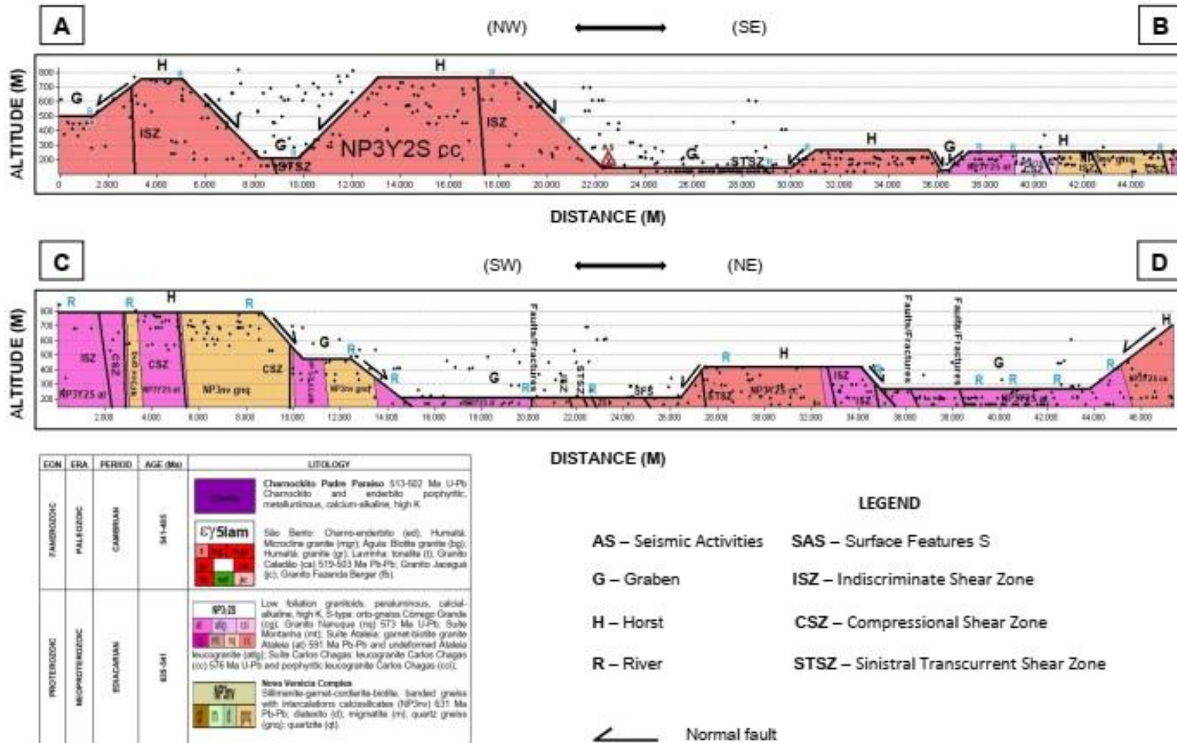
Figure 12 – AB (NW-SE) and CD (NE-SW) scan profiles
