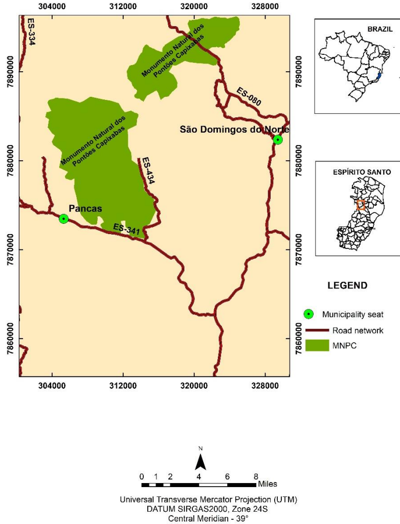
Figure 1- Location map of the studied area
