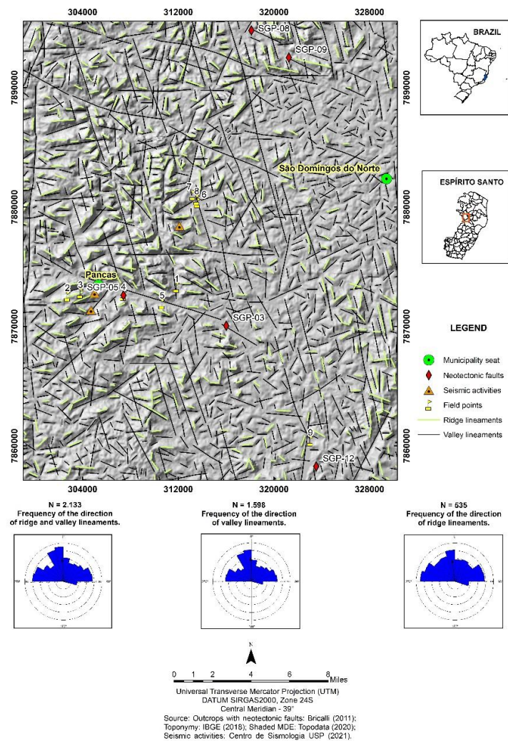
Figure 4 - Lineament map
