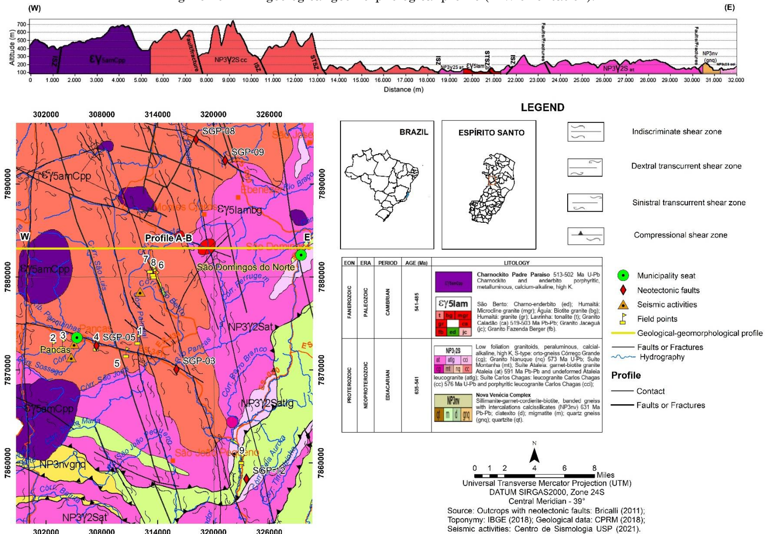
Figure 10 – A-B geological-geomorphological profile (E-W orientation).
