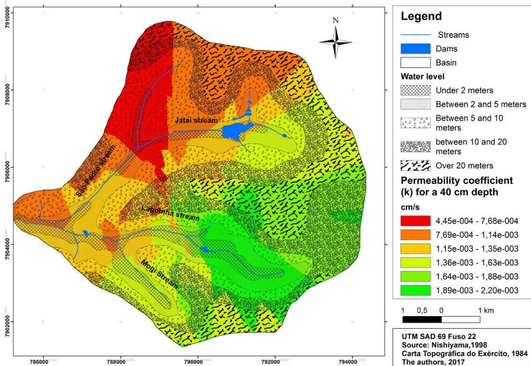
Figure 11. Groundwater level integrated to the coefficient of permeability (k) for the 40 cm depth.
