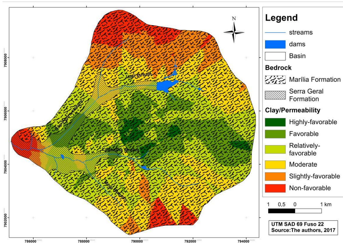
Figure 10. Areas with the possibility of infiltration. Rendered by the integration of the clay fraction percentages with the coefficient of permeability at a 40cm depth, both overlapping the bedrock.
