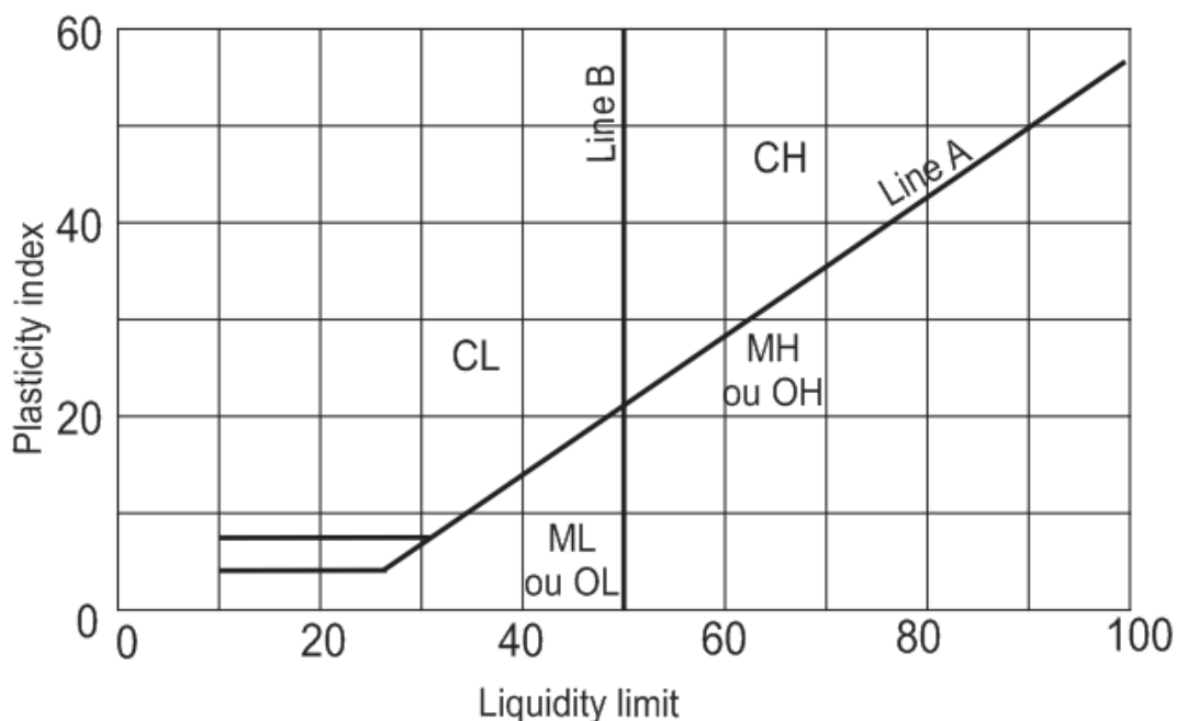
Figure 2. Plasticity Diagram.
