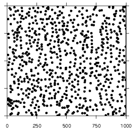
Fig. 1 – Spatial pattern of very large trees in sample block #1. Plot area covers 1000 x 1000 m = 100 ha.
