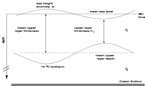
Fig. 1 - Schematics of the two-layer reduced gravity approximation, with an upper layer of mean density \rho_1 , thickness h that extends to the depth of the 10°C isotherm and a lower layer with mean density \rho_2 . The ocean surface has a sea height anomaly \eta^1 .
