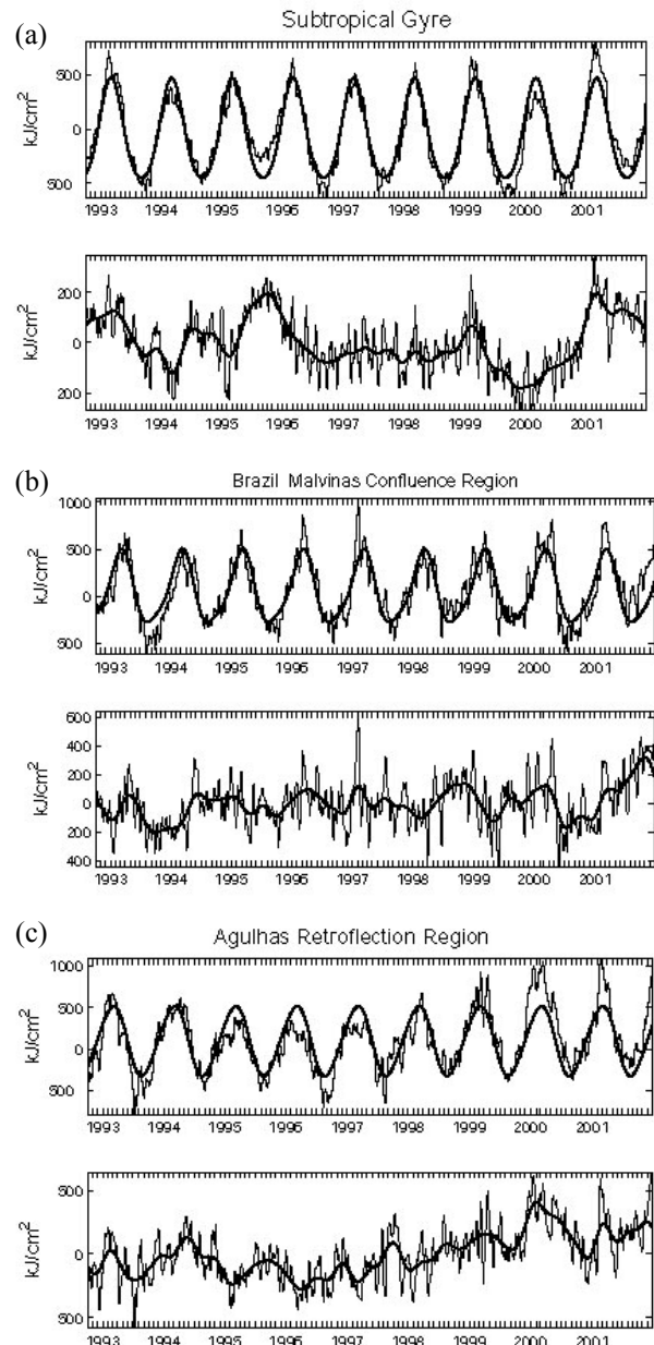
Fig. 5 - Each panel has two plots. Top plot: Thin line: Average upper layer heat content (HCA); Thick line: Annual plus semiannual cycles for the Average upper layer heat content. Bottom plot: Thin line: Upper layer heat content minus annual plus semiannual cycles; Thick line: The same as the black line but filtered.
