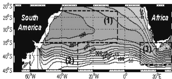
Fig. 3 - Contours (in meters) of the climatological upper layer depth referenced to the 10°C isotherm. Three regions are indicated: (1) The Subtropical Gyre; (2) The Brazil-Malvinas Confluence Region; (3) The Agulhas Retroflection Region
