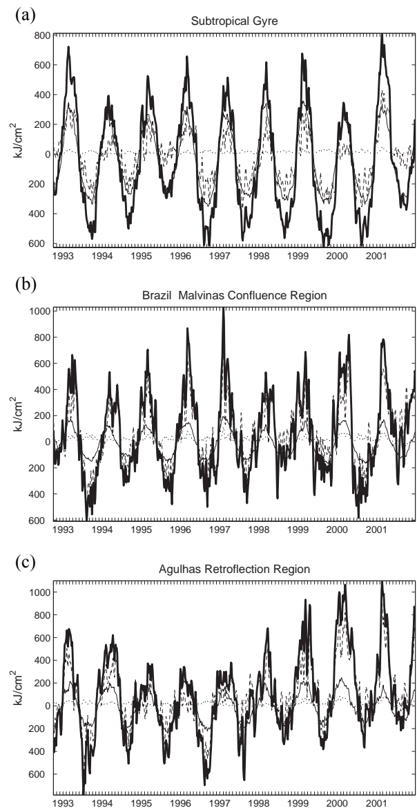
Fig. 4 – Solid thick line: Upper layer heat Content (HC); Solid thin line: First term in (9); Dotted line: Second term in (9); and Dashed line: Third term in equation (9), averaged on each one of the regions indicated in Fig. 3.
