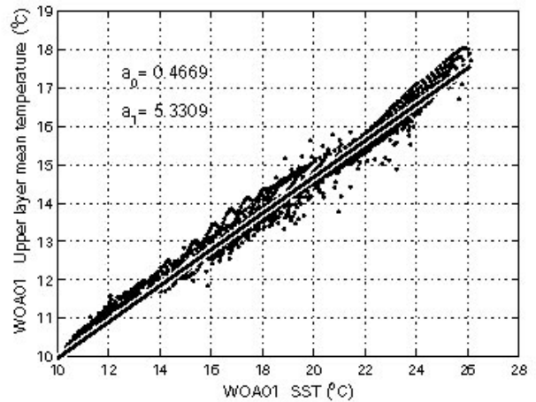
Fig. 2 - Linear regression between SST and upper layer mean temperature calculated from WOA01. The scatter plot contains all data points in the region 45S-19S, 70.5W-30.5E.
