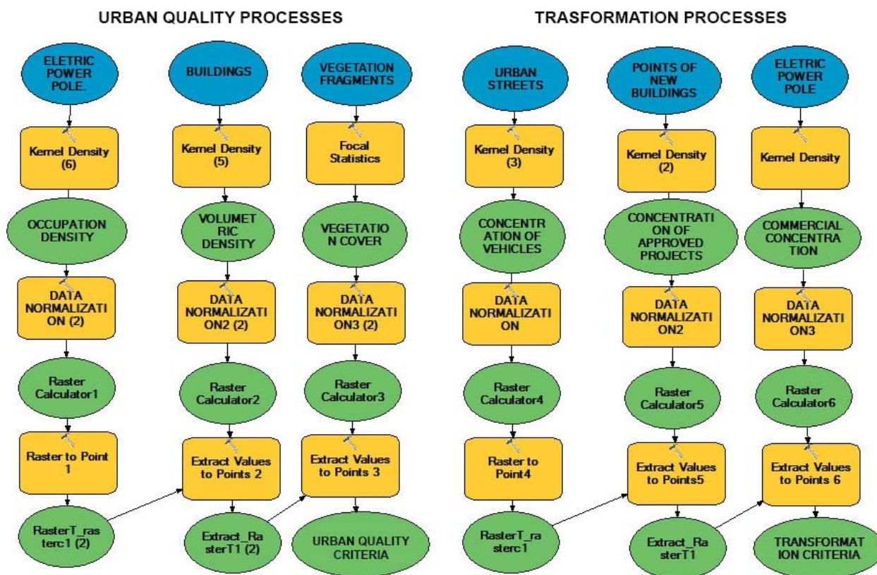
Fig. 3 - Process Models in ESRI ArcGIS's Model Builder. Ellipses represent datasets, while rectangles represent processing functions.
