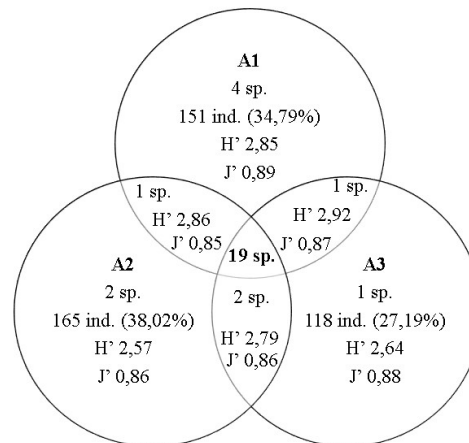
Figure 6. Venn diagrams containing unique and common species to each environment, as well as the number of individuals, diversity index of Shannon-Weaver ( H' ) and Pielou equability ( J' ), sampled in the Mata da Frascalli, Rio Largo, Alagoas, Brazil (A1 - fragment edge, A2 - 30m from the edge and A3 - 70m from the margin).
