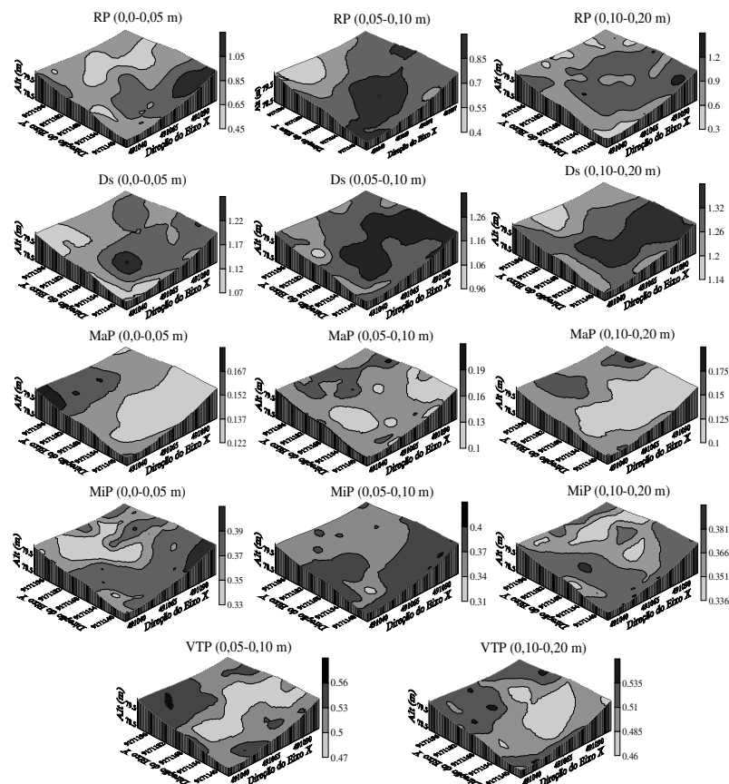
Figure 2. Kriging maps of soil physical attributes in forest at different depths.
