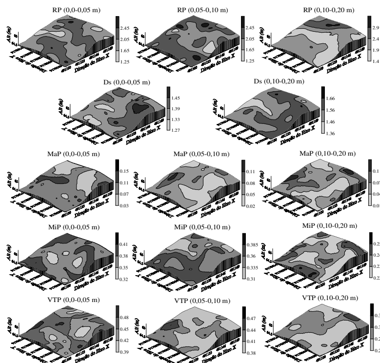
Figure 1. Kriging maps of soil physical attributes in natural grasslands at different depths.
